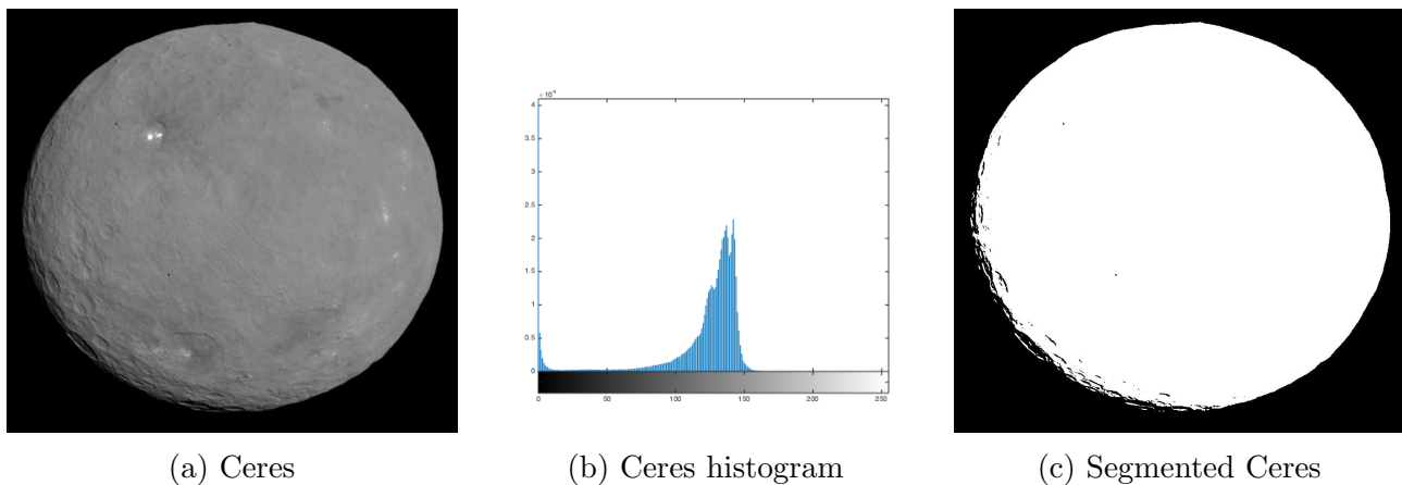
Figure 1: Ceres
