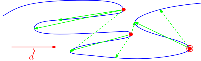
Figure 6: Occulters for the direction d in red. Green arrows represent backpaths: the length of the plain arrows is to be checked, whereas we know that the backpaths represented by dashed arrows are not the longest ones.
